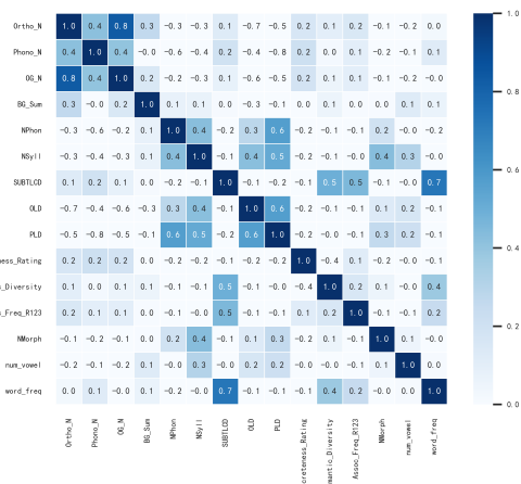
Figure 18: Correlation of Attributes
